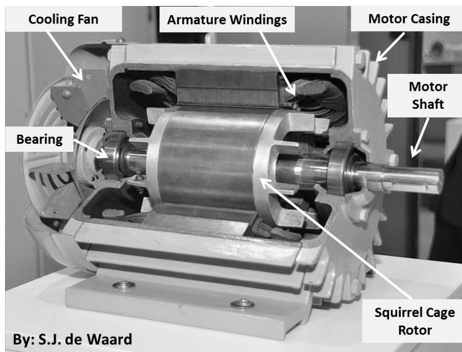
Figure 2.5: AC induction motor construction.
