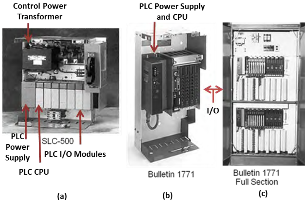
Figure 3.21: PLC's incorporated into an Allen-Bradley MCC.
